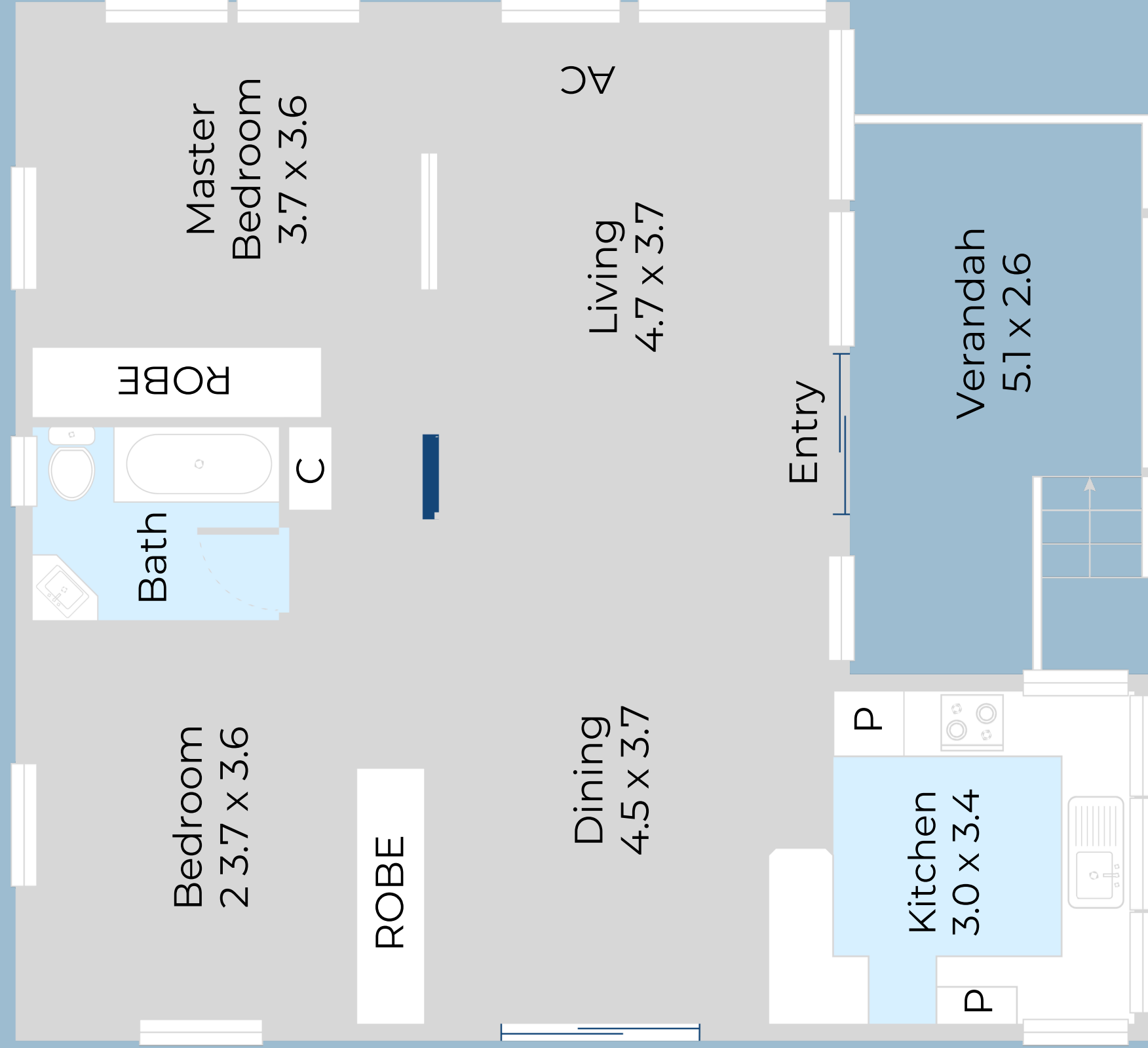
Trebetha Cottage Floor Plan
